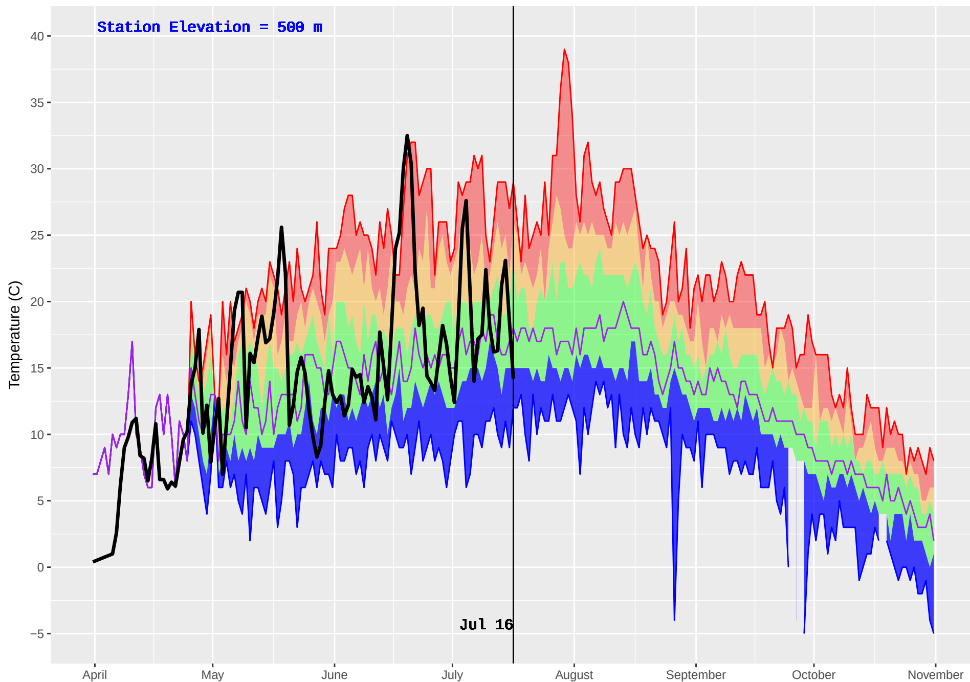
CRANBERRY (433) : Historical (1995–2016) and Current (2018) Daily Temperature
