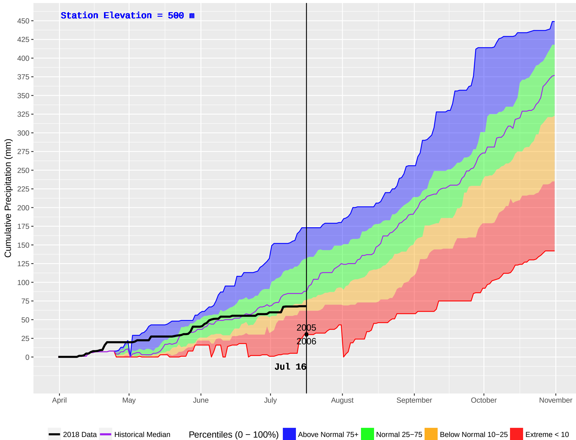
CRANBERRY (433) : Historical (1995–2016) and Current (2018) Daily Cumulative Precipitation
