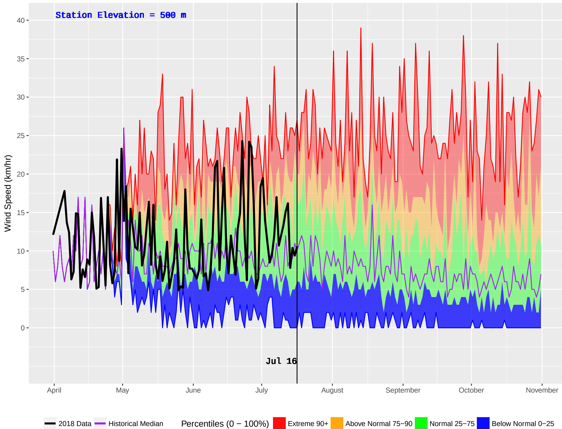
CRANBERRY (433) : Historical (1995–2016) and Current (2018) Daily Wind Speed
