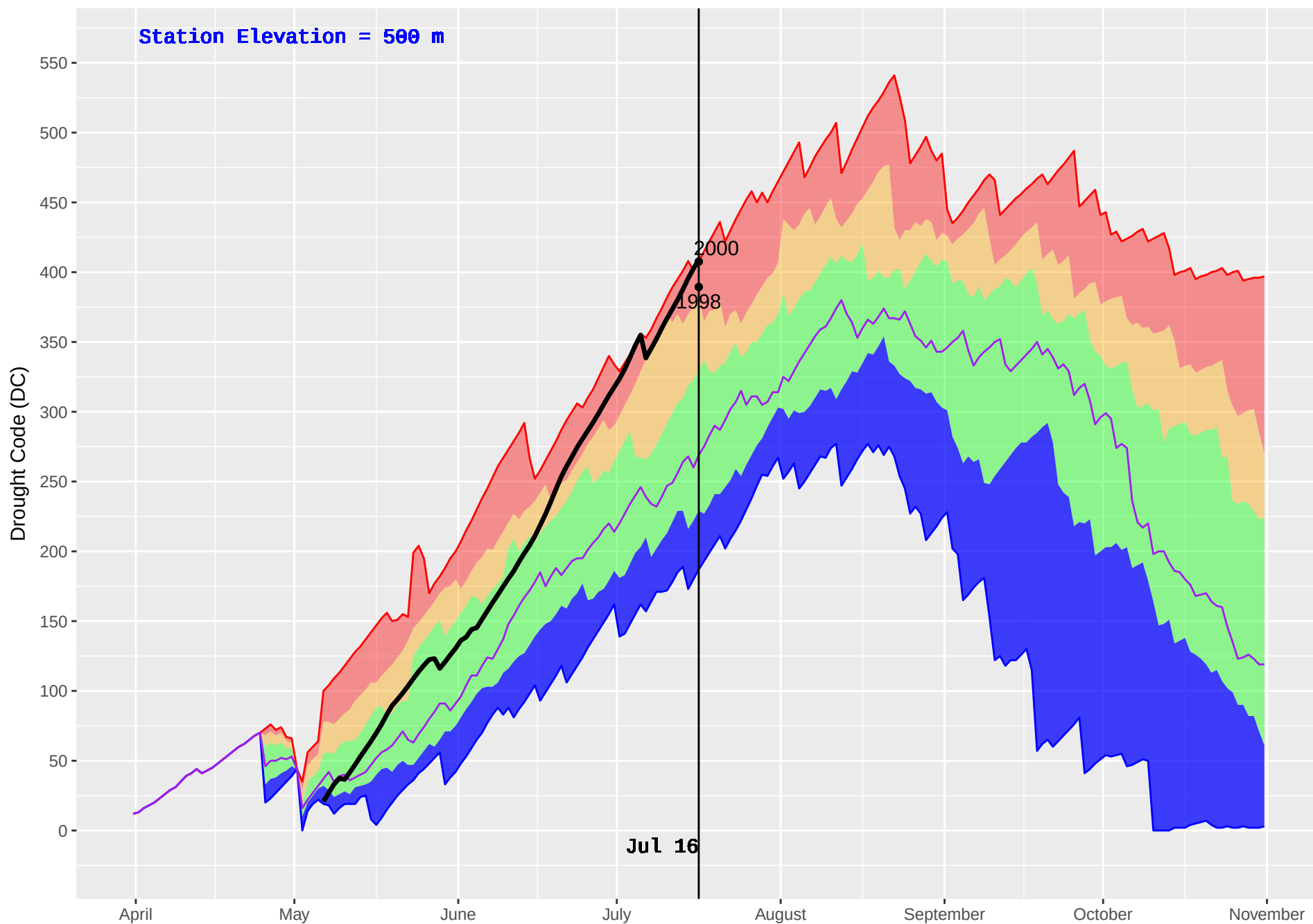
CRANBERRY (433) : Historical (1995–2016) and Current (2018) Daily Drought Code (DC)
