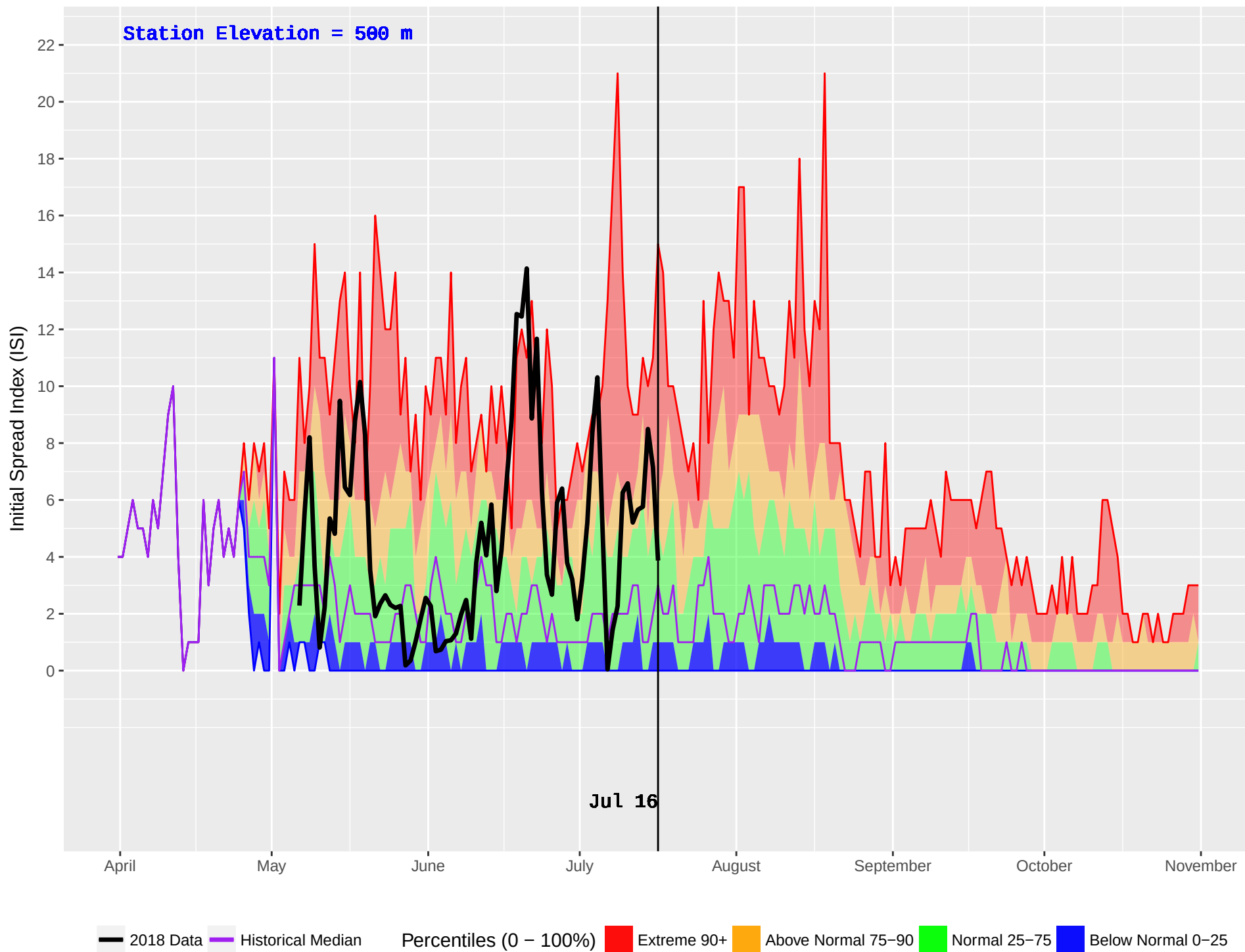
CRANBERRY (433) : Historical (1995–2016) and Current (2018) Daily Initial Spread Index (ISI)
